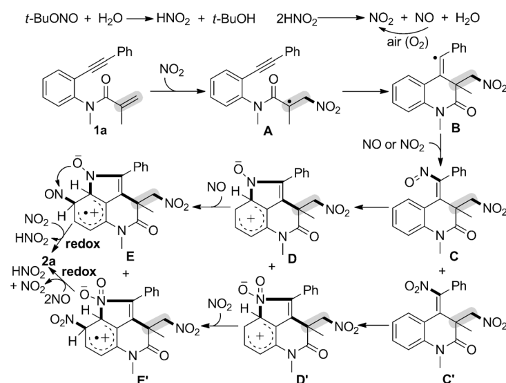
Scheme 2. Possible mechanisms.
